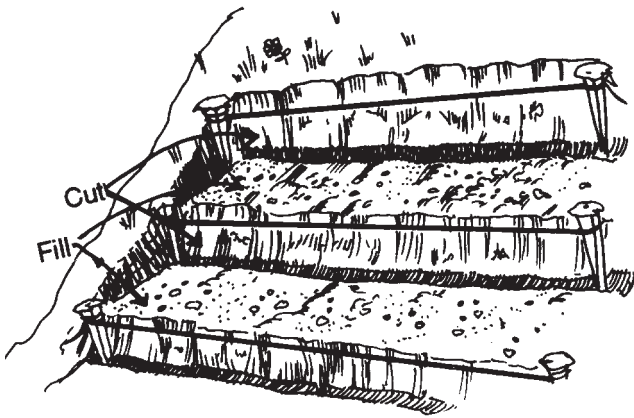
Terrace Layout
